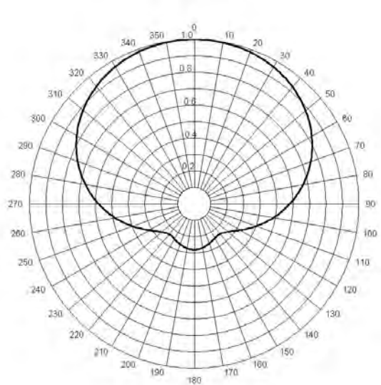
JFVX Single Dipole Pattern
