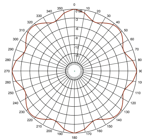
Standard 4 Around Omni Azimuth Pattern
